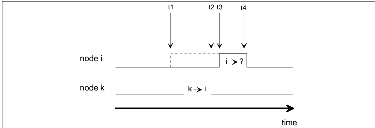
Figure 15 ring messages from the nodes i and k on an asynchronous bus t_1 The timer T_{Typ} in node i has elapsed and the ring message of node i is released for transmission. As the bus is busy, this ring message cannot be transferred. t_2 Node i receives the respective ring message from node k. t_3 The ring message of node i is transmitted to the bus. t_4 The ring message of node i was transmitted to the bus successfully.
